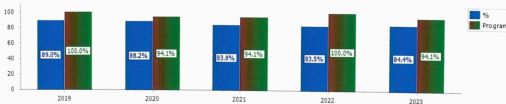
Program vs Total Pass Percentage
